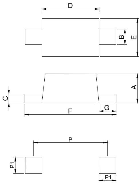
Land Pattern
