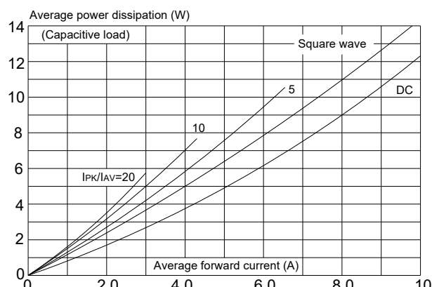
FIG.5: Power dissipation
