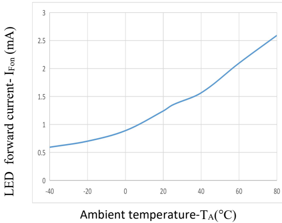
Fig.5 LED Forward current vs. Ambient temperature characteristics
