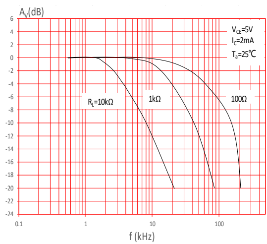
FIG.10: Frequency Response
