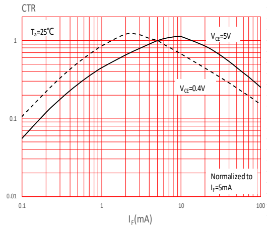
FIG.6: Normalized Current Transfer Ratio vs. Forward Current
