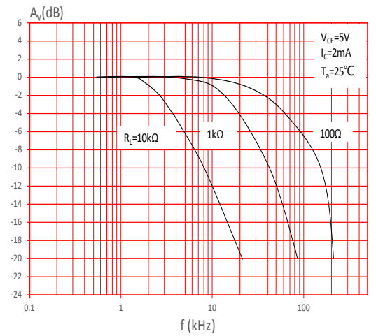
FIG.10: Frequency Response
